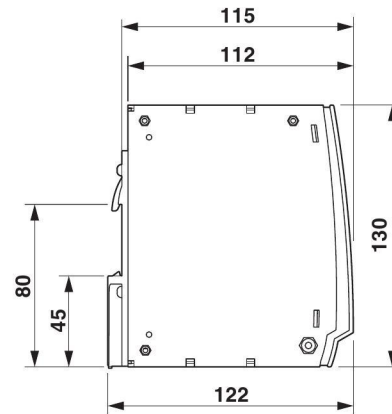
Figure 3 Device dimensions
