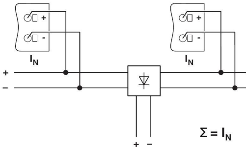
Figure 44 Redundancy operation with decoupling via diode module
