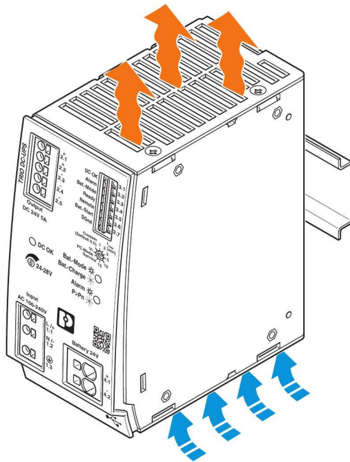
Figure 5 Convection
