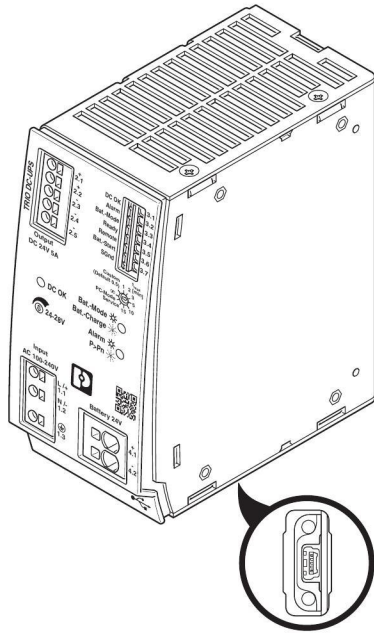
Figure 40 USB interface MINI type B (bottom of device)
