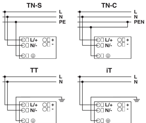
Figure 16 Network types
